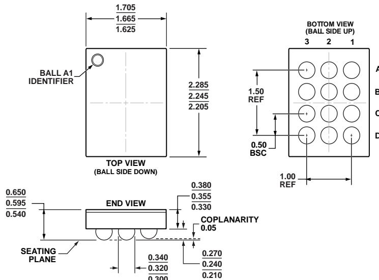
Figure 78. 12-Ball Wafer Level Chip Scale Package [WLCSP] (CB-12-9)
